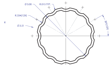
3" DIAMETER FLUTED
