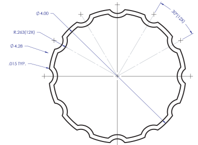
4" DIAMETER FLUTED
