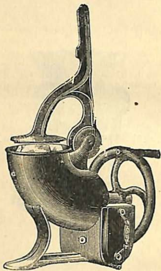
ROTARY ICE SHAVER
