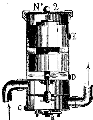
Regulator.
