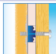
Insulated Plasterboard
