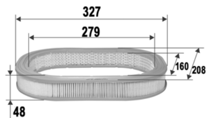
Valeo 585722
