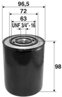
Valeo 586007
