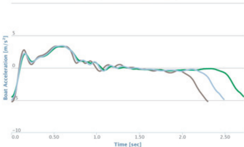
Typical Stroke Boat-acceleration
