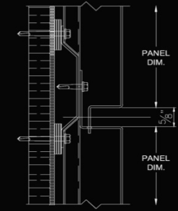
HORIZONTAL JOINT DETAIL RAIN SCREEN 100
