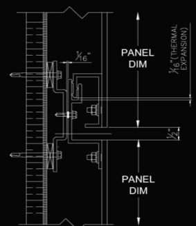
HORIZONTAL JOINT DETAIL RAIN SCREEN 400
