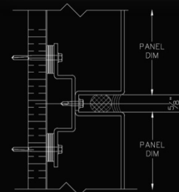
HORIZONTAL JOINT DETAIL BARRIER SYSTEM 100
