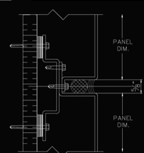
HORIZONTAL JOINT DETAIL BARRIER SYSTEM 200
