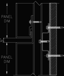
HORIZONTAL JOINT DETAIL RAIN SCREEN 300
