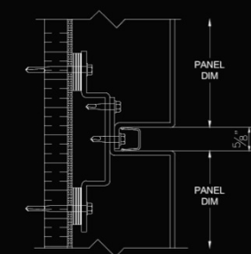
HORIZONTAL JOINT DETAIL RAIN SCREEN 200
