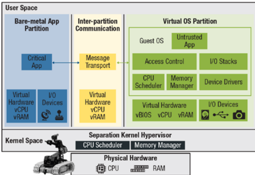
איור 2 A separation kernel hypervisor (SKH) is designed to isolate hardware resources and host software and guest operating systems in independent partitions, and to control information flow between all hardware components and partitions.
