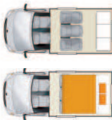
Apollo Vivid: dag- & nacht-layout
