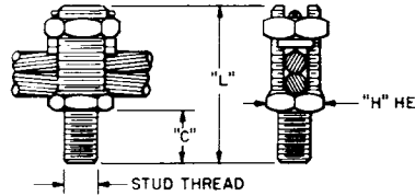
FIGURE 2 TYPE K2S FOR TWO WIRES
