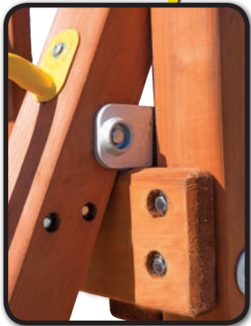
Ladder Safety Bracket
