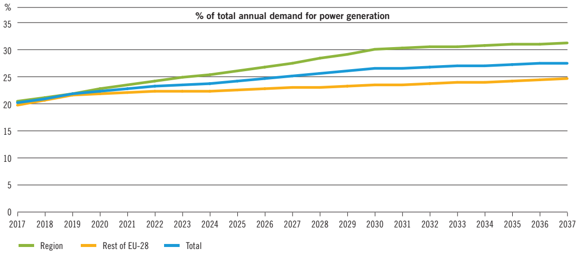
Figure 3.18: Evolution of the share of total demand used for power generation between 2017 and 2037 according to the Blue Transition scenario (Source: projection based on data from TSOs collected by ENTSOG)
