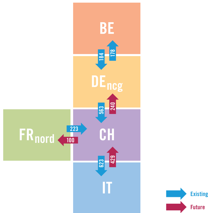
Figure 6.6: Schematic representation of the South-North Corridor and related existing and future capacities in GWh/d (Source: ENTSOG Capacity Map 2016 for existing capacities, TSO promoters for future reverse flow capacities)
