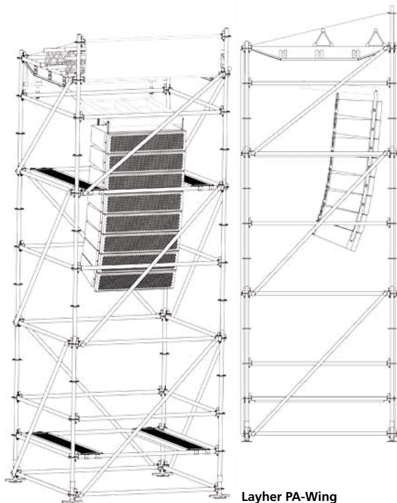
Layher PA-Wing
