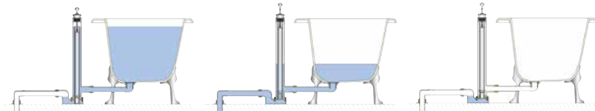
Full bath using overflow
