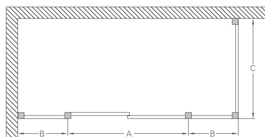
Sliding door with in-line and side panel
