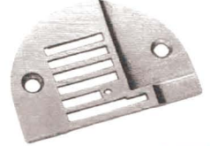
6 ROW NEEDLE PLATE FOR SINGLE NEEDLE LOCKSTITCH #NP-6B
