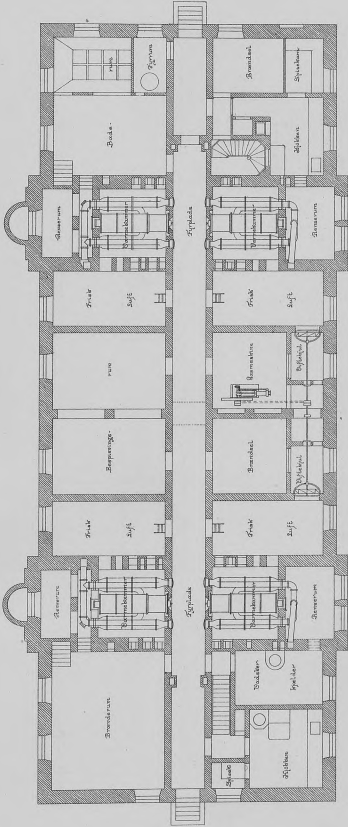
Plan of the building
