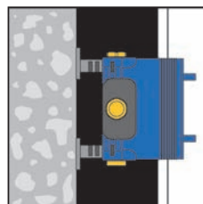
In-front-of-wall installation.
