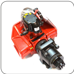
Part No: FA0725 Coupling VBG 575V-2 VBG Part Number: 09-070100
