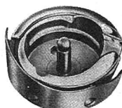
HOOK #91-064661-91
