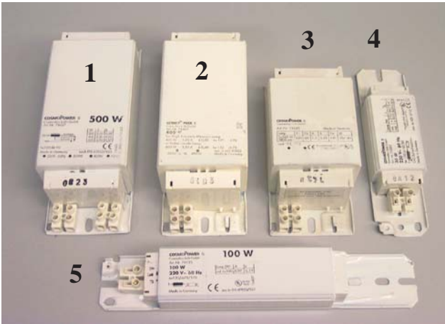
Choke Ballasts
