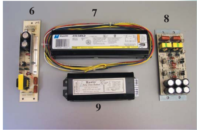
Electronic Ballasts
