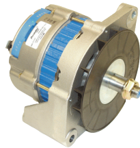
Alternator To Fit: ERF / FODEN 1012219, 1036120, 1066152, 1334212R, 6200596000, Z05815902, Z6200914000
